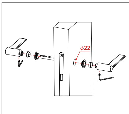
Solo maniglia Handle only
